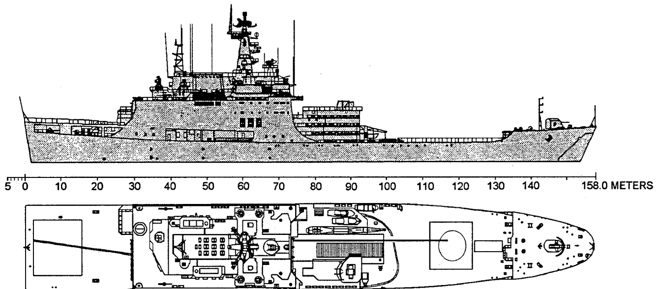
Figure 6-22.—IVAN ROGOV-class LPD.
